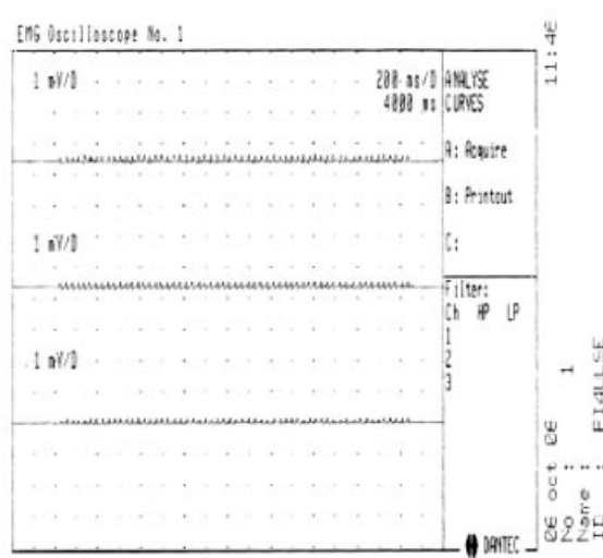
Fig. 3. The effect of lidocaine on TASER® X26-induced EMG recorded on right (top tracing), left (middle tracing) hind limbs and left front limb (bottom tracing). The electrodes were placed in the intercostical space at right side. Lidocaine was injected into the subcutaneous tissue around the electrodes.
